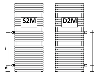
Specificare "i" e "d" i min = 5cm d min = 2cm
