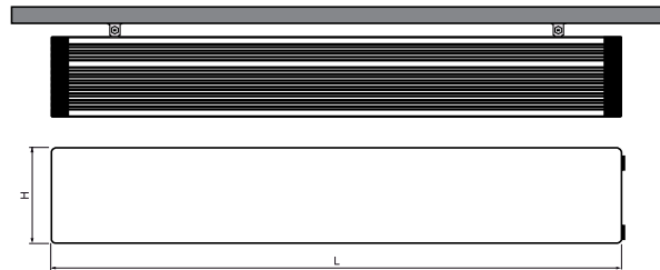
T33 | Top view
