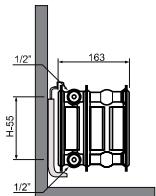
T33 | Side view
